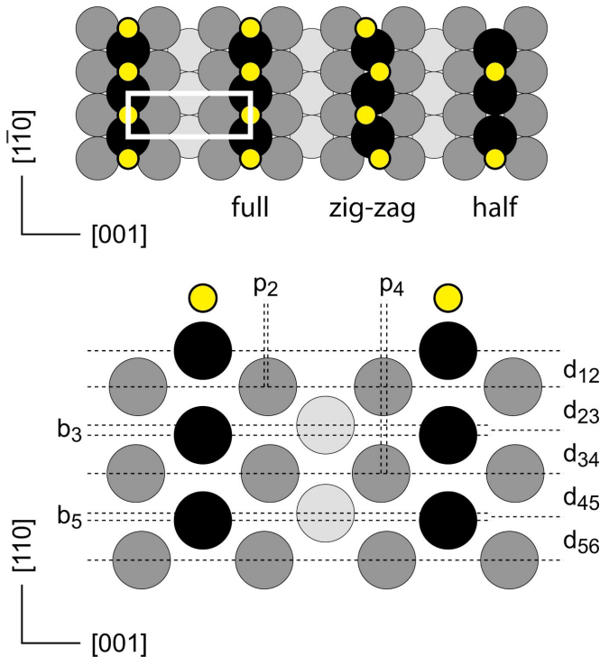
FIG. 2. (Color) Model of the Pt atom geometry on clean and hydrogen-modified H/Pt(110)( 1 \times 2 ) surfaces with structural parameters determined. Typical H atom (yellow) arrangements used in the DFT calculations are denoted as full ( \beta_2 -H), zig-zag (slightly distorted \beta_2 -H to elucidate the effects of low energy lateral H displacements), and half (half-filled \beta_2 -H), respectively.
